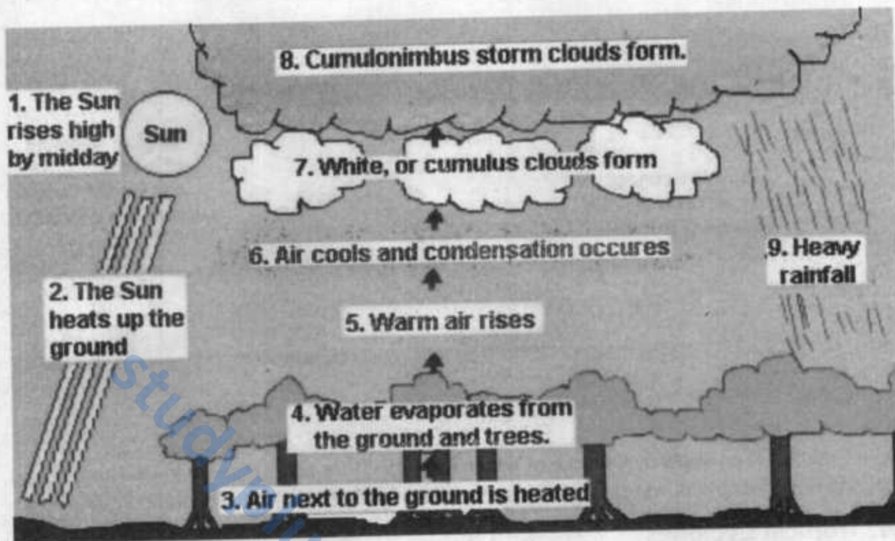
Convectional rainfall
